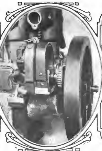
Fig. 12—Magneto upon a ledge of motor casting and method of holding same in position
